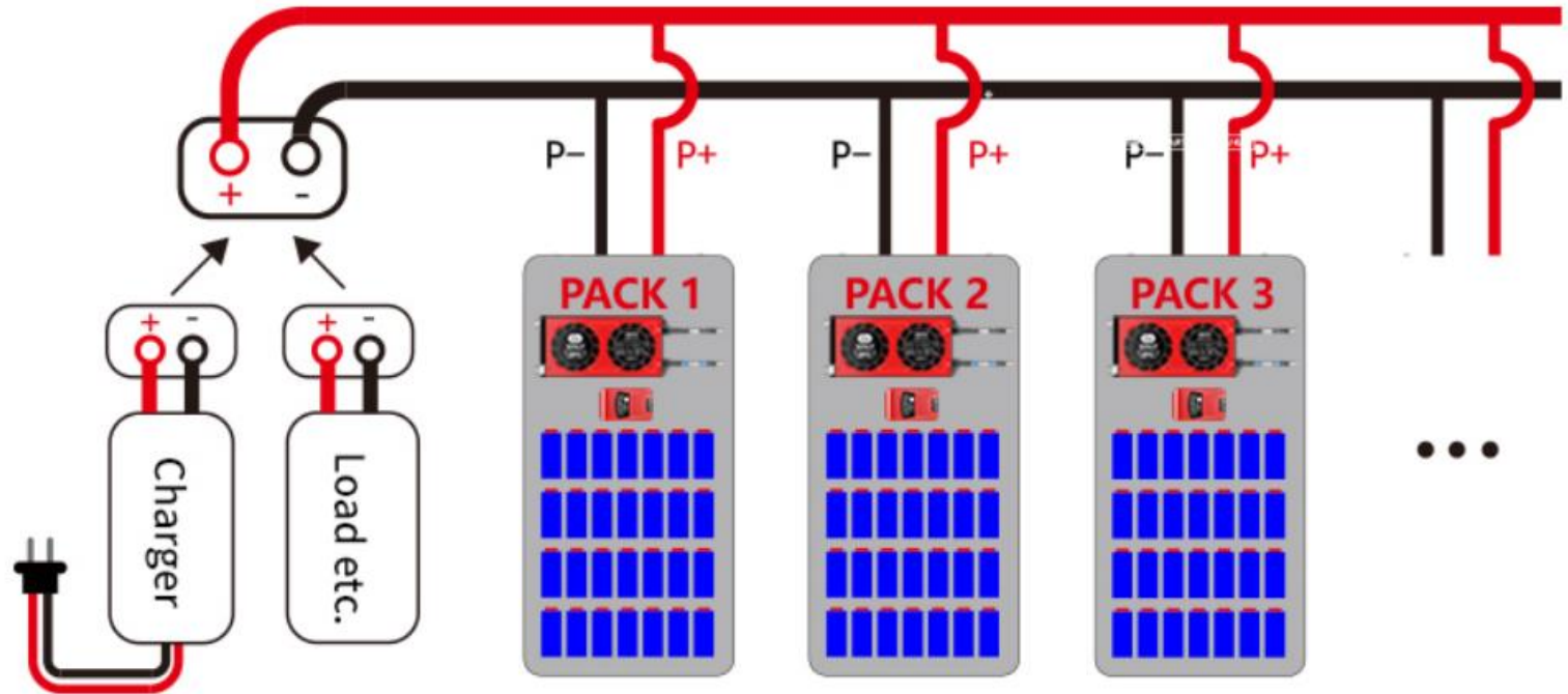
PACK parallel battery pack wiring diagram:
