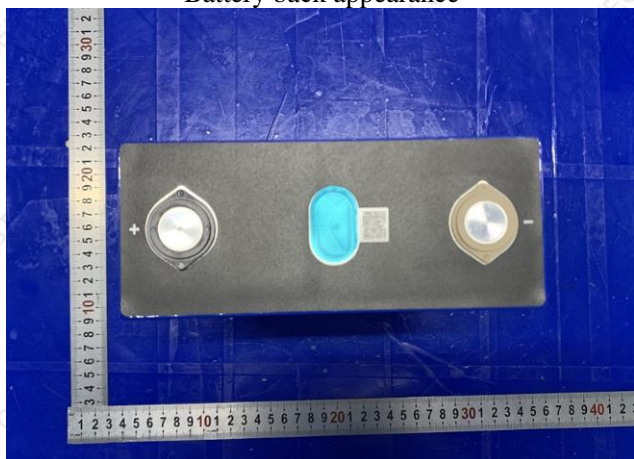
电池背面外观 Battery back appearance
